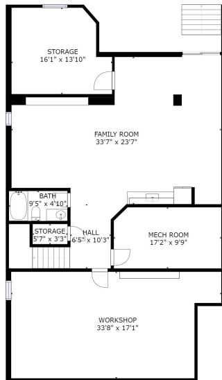
LOWER LEVEL
